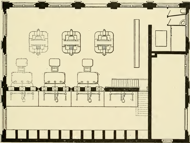
Fig. 168. Plan of Substation of West Shore Railroad
